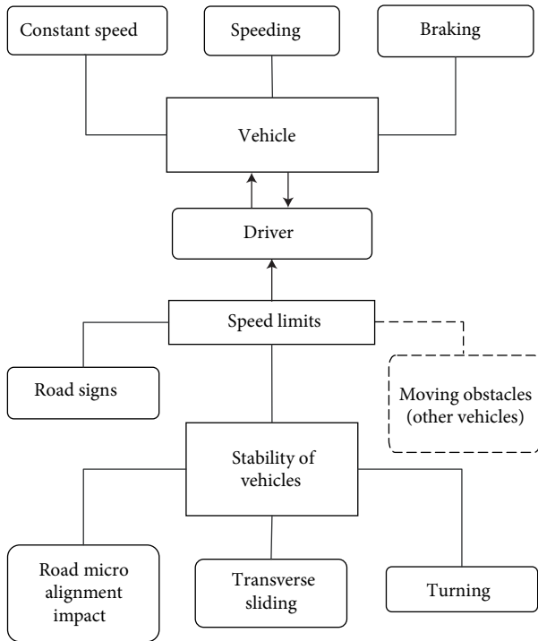
Fig. 6. Principle scheme of the system driver-vehicle-road when constructing a complex model of a vehicle's motion on a road
